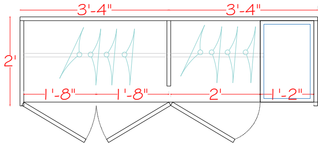
DRESSER WARDROBE PLAN
