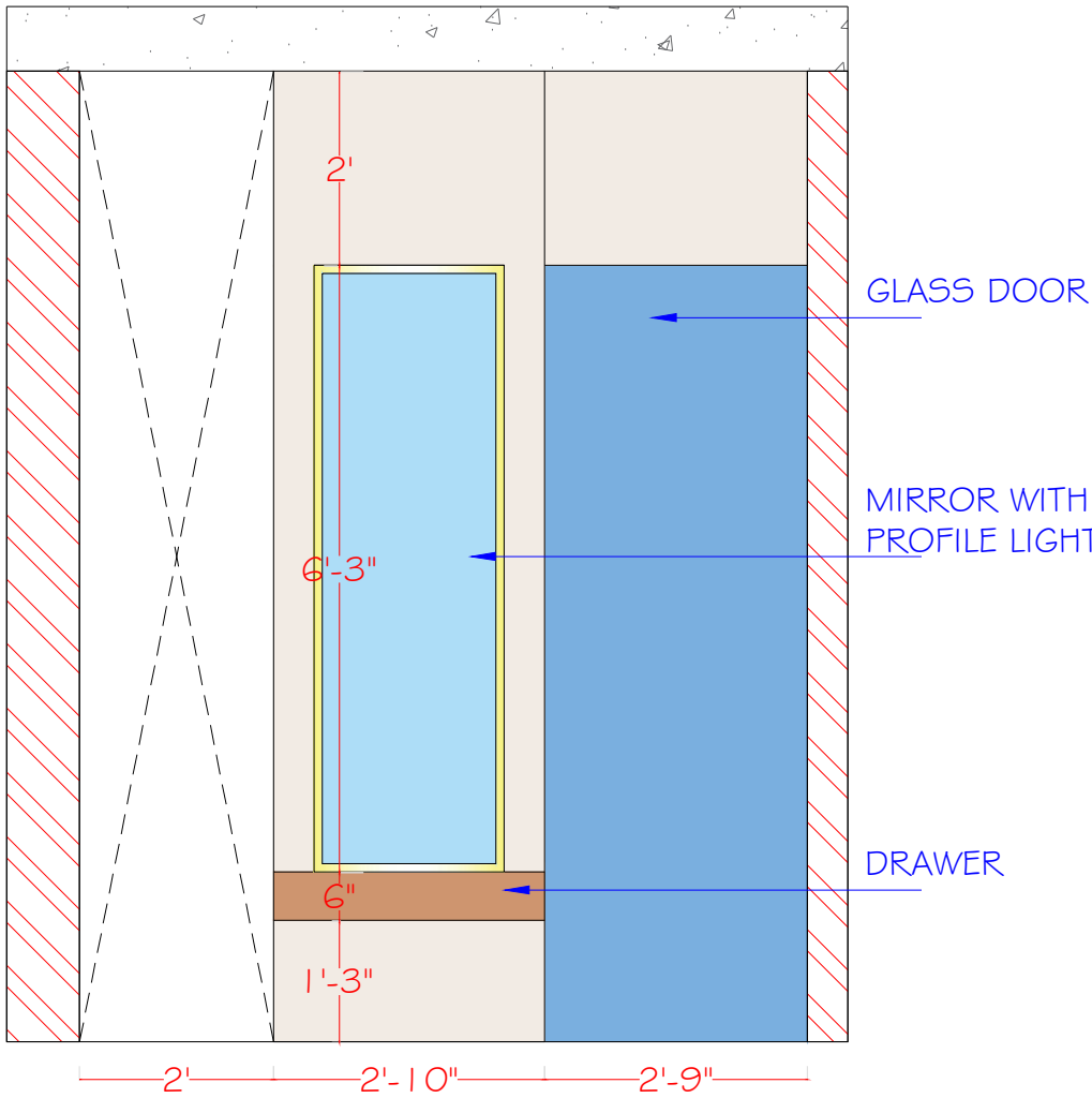
WALL ELEVATION A
